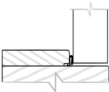
Timber – Full Width planted stop
